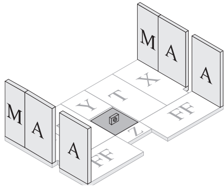
Fig. 9b– Step 2, Side Firebrick Installation Four (4) A-Size; Two (2) M-Size
