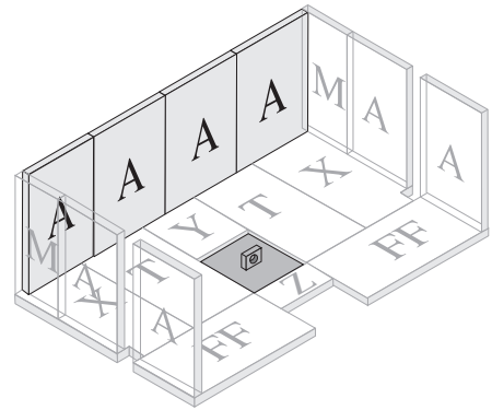
Fig. 9c– Step 3, Back Firebrick Installation Four (4) A-Size
