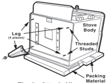
Fig. 2– Attach (4) Legs
