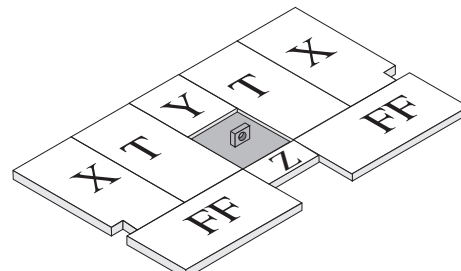
Fig. 9a– Step 1, Bottom Firebrick Installation Two (2) FF-Size; Two (2) T-Size; Two (2) X -Size; One (1) Y-Size; One (1) Z-Size
