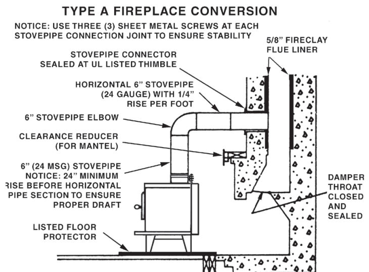
Fig. 14 - Fireplace Conversion
