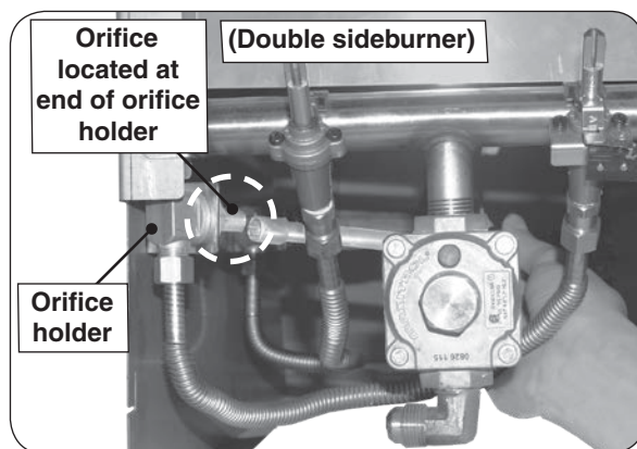
Fig. 32-2 Double sideburner orifice locations
