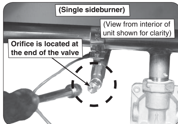
Fig. 32-1 Single sideburner orifice location
