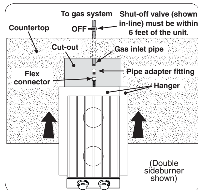
Fig. 19-4 Household propane & nat. gas diagram
